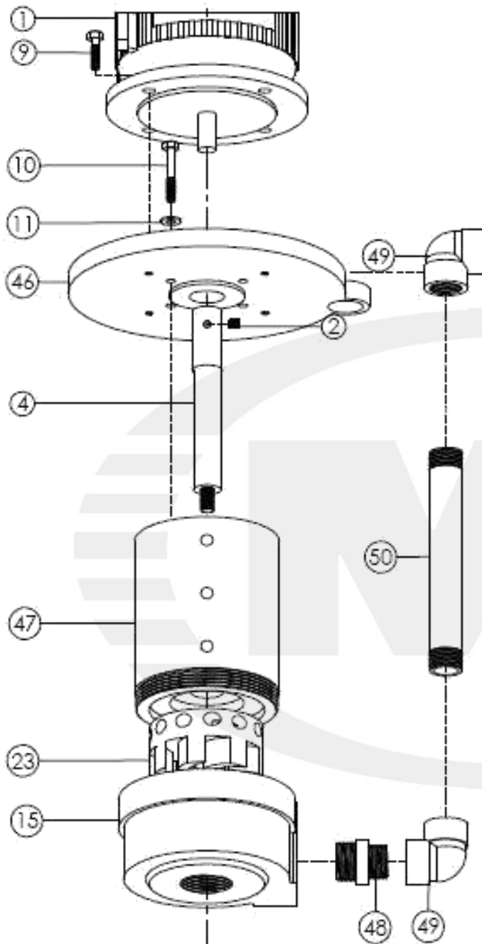
Bomba Master S 10-10/S 10-15
